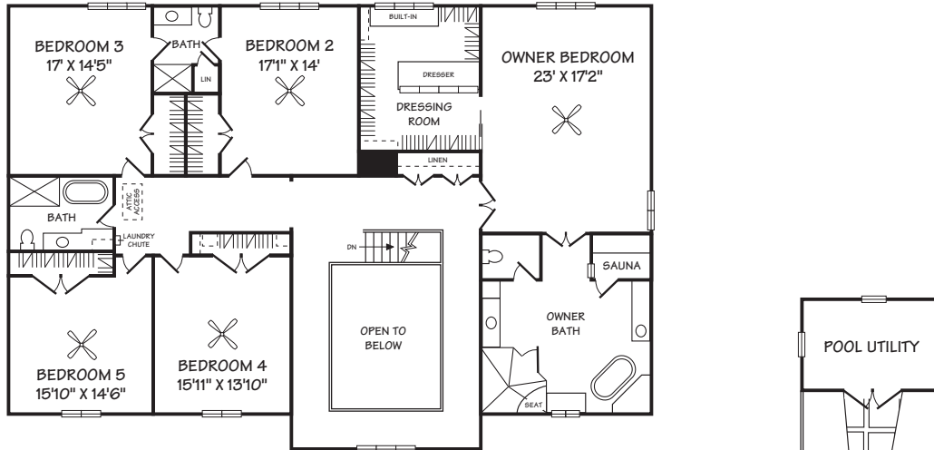
SECOND LEVEL 8'1" VAULTED CEILING
